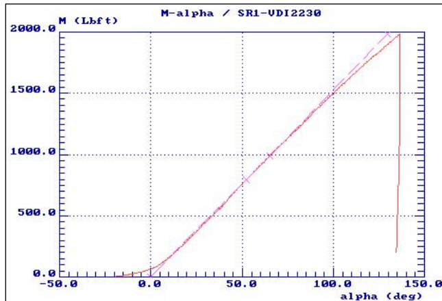
Figure 31. Torque-Angle Signature with Embedment
